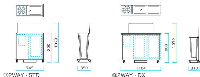
⑦ 2WAY・STD
